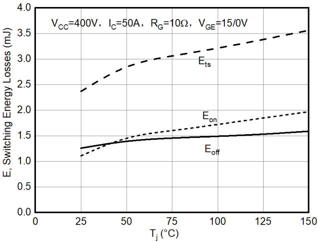
Figure 15. E_{on} , E_{off} as a function of T_j
