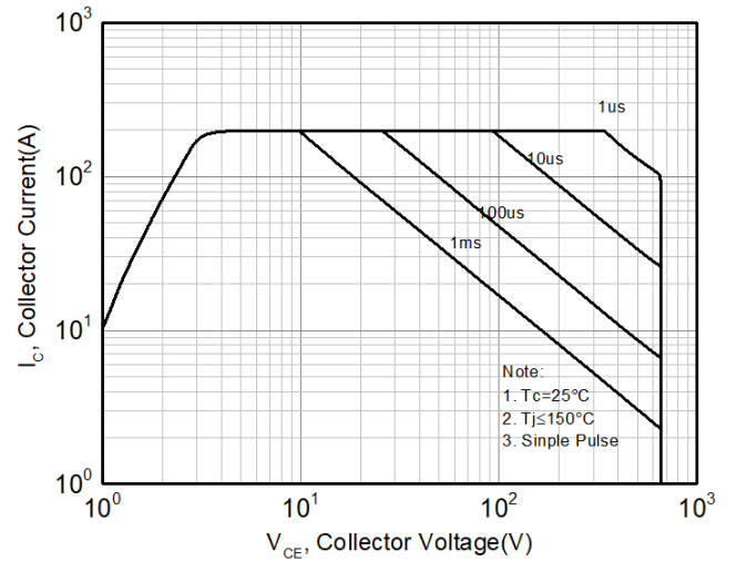
Figure 16. FBSOA
