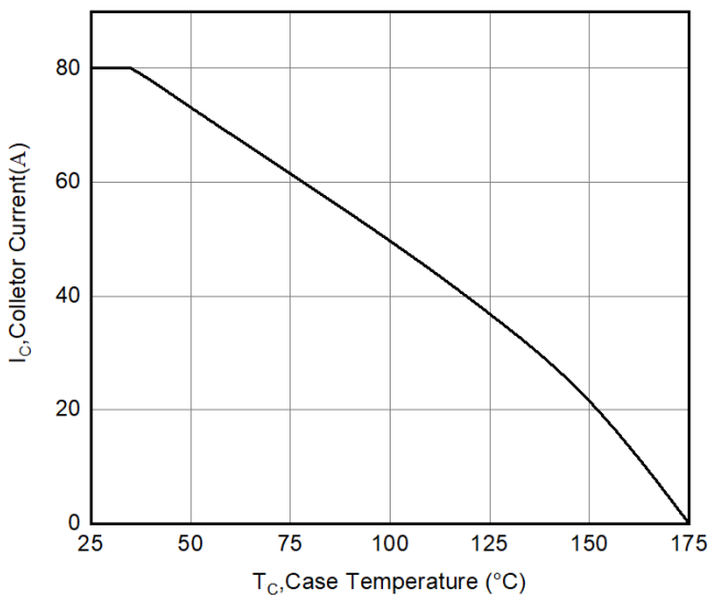
Figure 17. Collector current as a function of case temperature ( V_{GE} \geq 15V , T_j \leq 150^{\circ}C )
